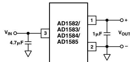
Figure 3. Typical Connection Diagram
