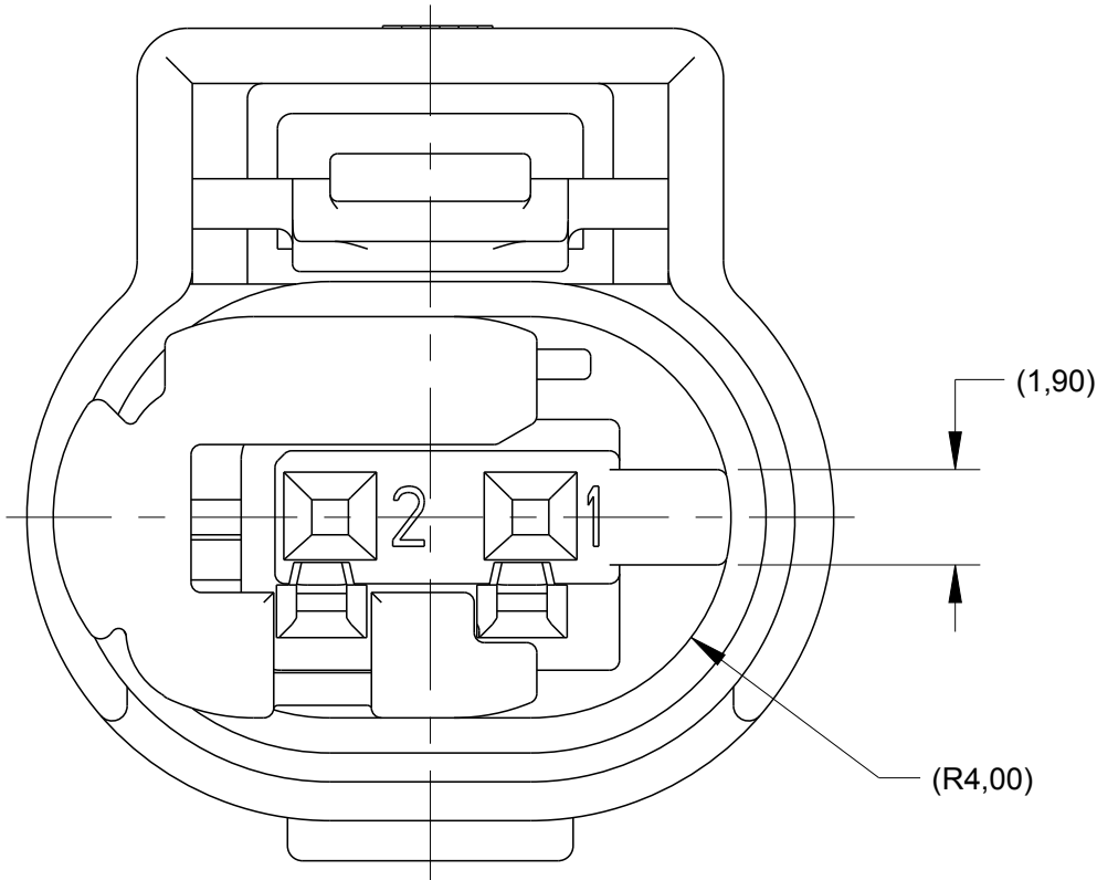
KEY CODE A 1-1438608-1 AND 1-1438608-5 AND 2-1438608-1 ONLY SCALE 6:1
