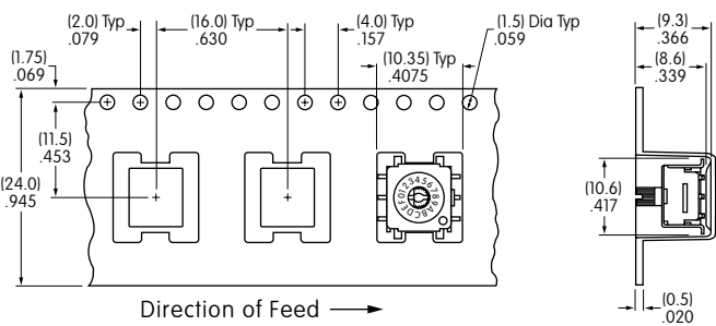
Tape Dimensions
