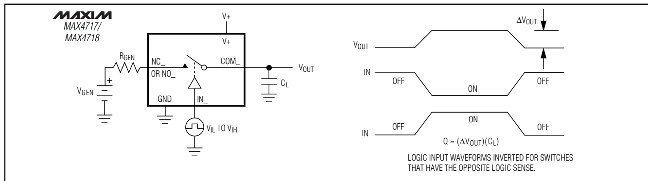
Figure 4. Charge Injection
