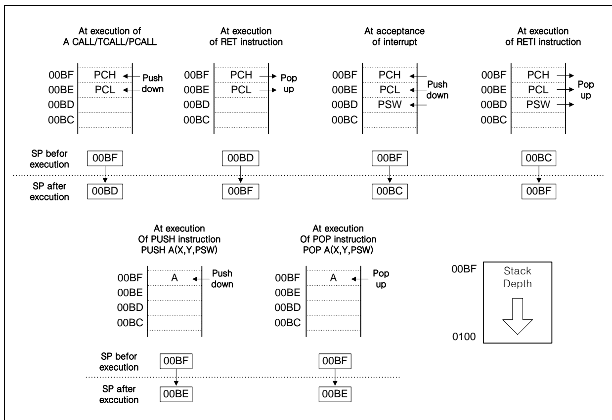
Figure 9-4 Stack Operation
