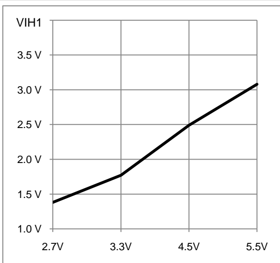
Figure 7-15 V_{IH1} - V_{DD}
