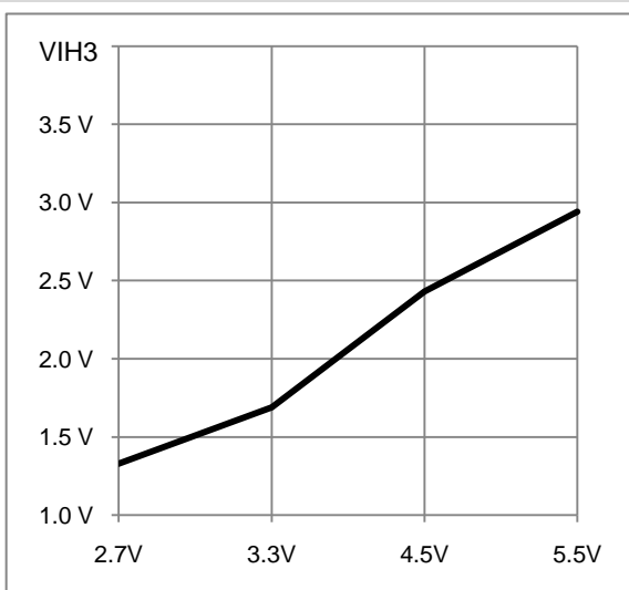
Figure 7-17 V_{IH2} - V_{DD}
