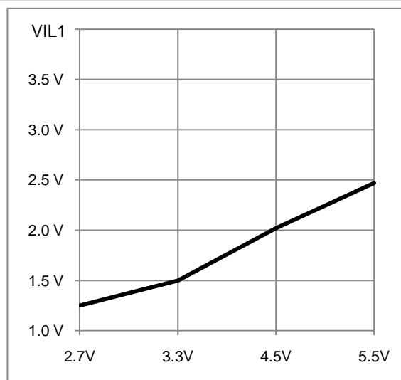
Figure 7-16 V_{IL1} - V_{DD}
