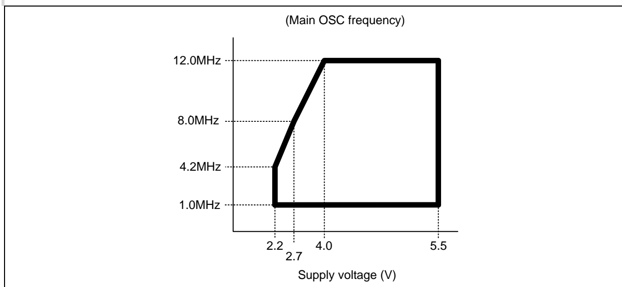
Figure 7-9 Operating Voltage Range
