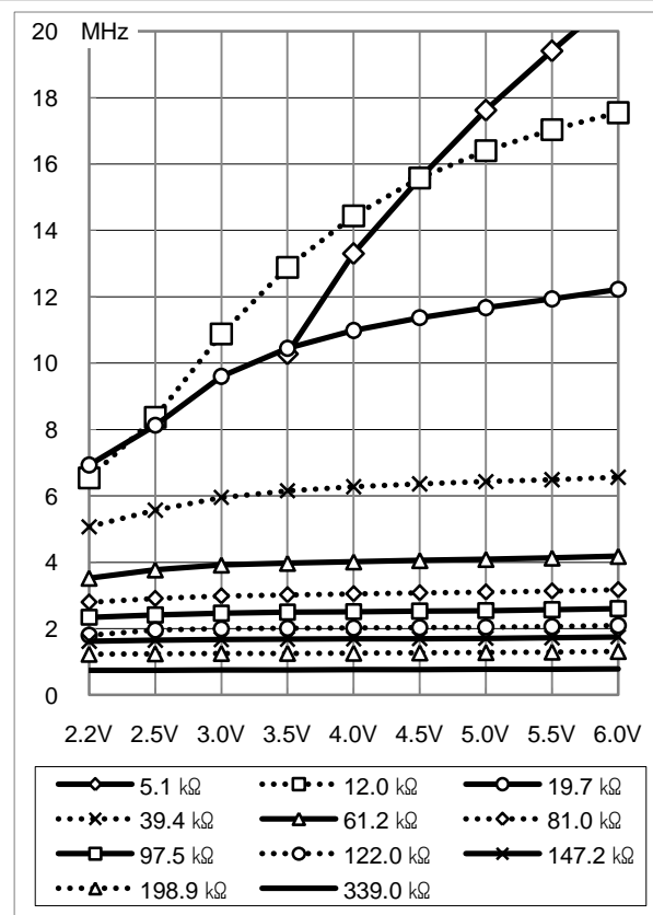
Figure 7-21 Ext. R/C OSC Freq. - V_{DD} at 85^{\circ}\text{C}
