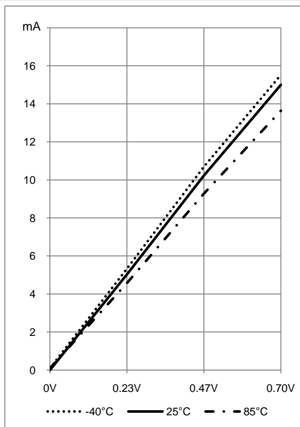
Figure 7-14 I_{OL} - V_{OL} at V_{DD}=5V
