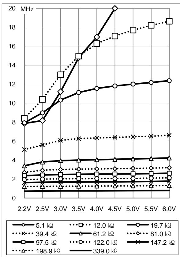
Figure 7-20 Ext. R/C OSC Freq. - V_{DD} at 25^{\circ}\text{C}
