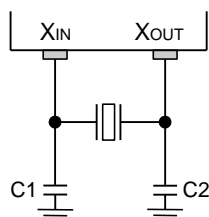
Figure 7-5 Crystal/Ceramic Oscillator
