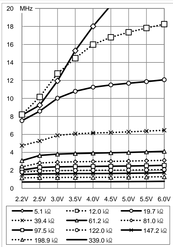
Figure 7-22 Ext. R/C OSC Freq. - V_{DD} at -40^{\circ}\text{C}
