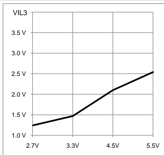
Figure 7-18 V_{IL2} - V_{DD}
