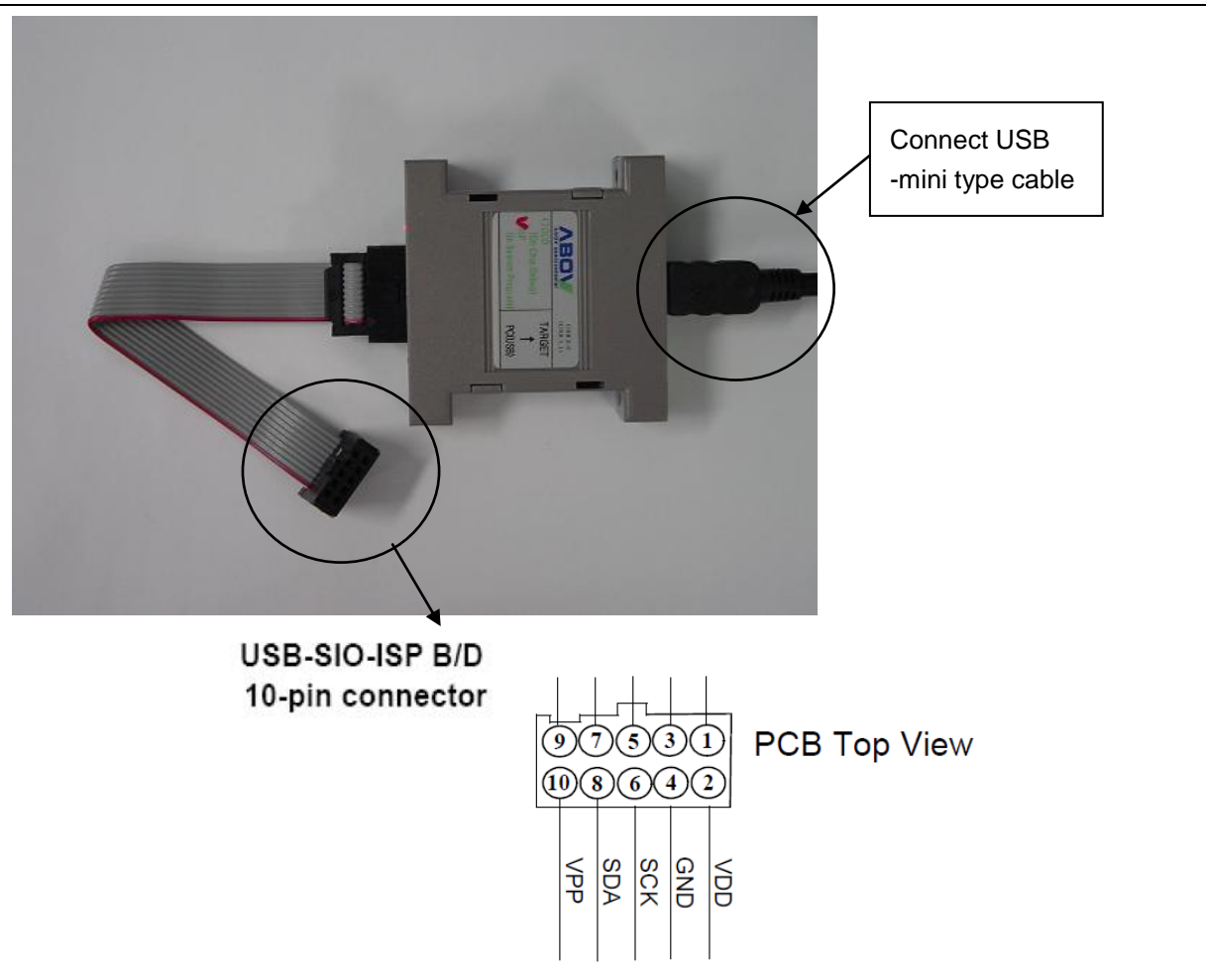
Figure 23-3 USB-SIO-ISP Board
