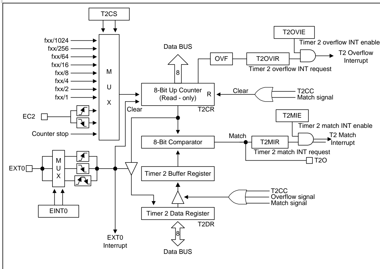
Figure 16-1 8-bit Timer 2 Block Diagram
