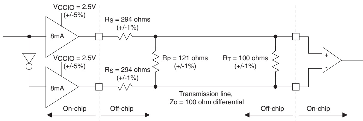
Figure 3-4. RSDS (Reduced Swing Differential Signaling)
