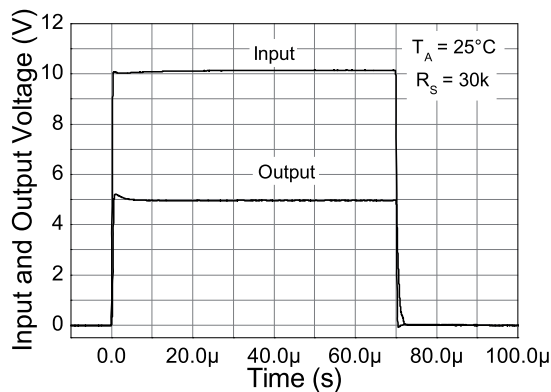
Long Pulse Response
