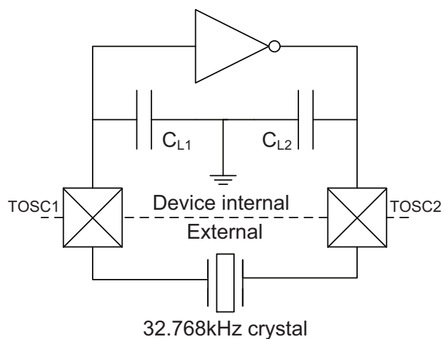
Figure 37-11.TOSC input capacitance.
