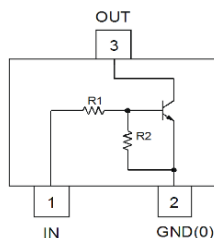
Device Schematic
