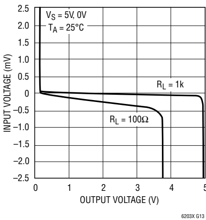
Open-Loop Gain
