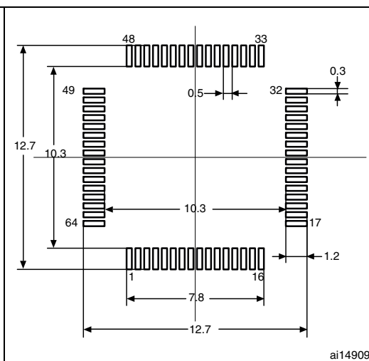
Figure 72. Recommended footprint (1)(2)
