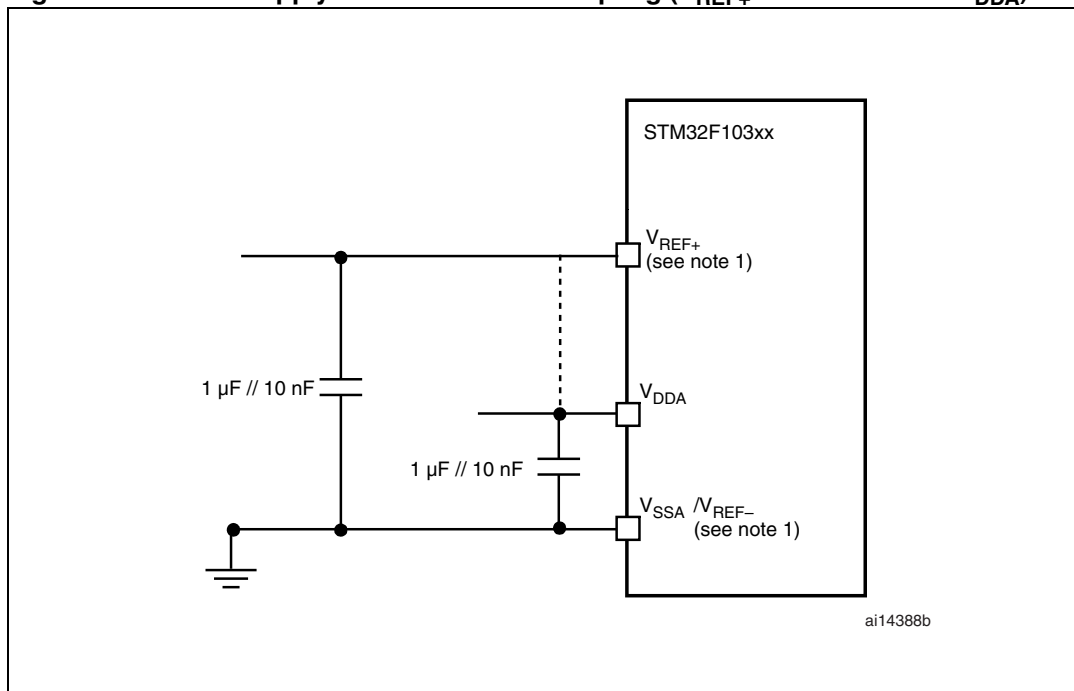
Figure 59. Power supply and reference decoupling ( V_{\text{REF}+} not connected to V_{\text{DDA}} )
