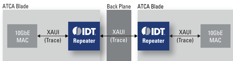
Figure 21: ATCA Application
