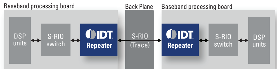
Figure 17: Wireless Systems with Backplanes
