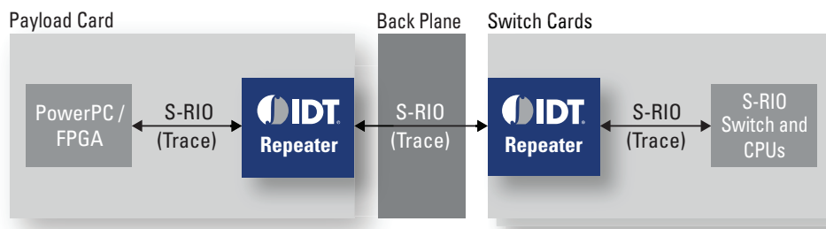
Figure 19: Military Application
