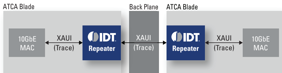
Figure 21: ATCA Application
