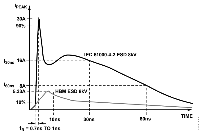
Figure 46. IEC 61000-4-2 ESD Waveform (8 kV) Compared to HBM ESD Waveform (8 kV)
