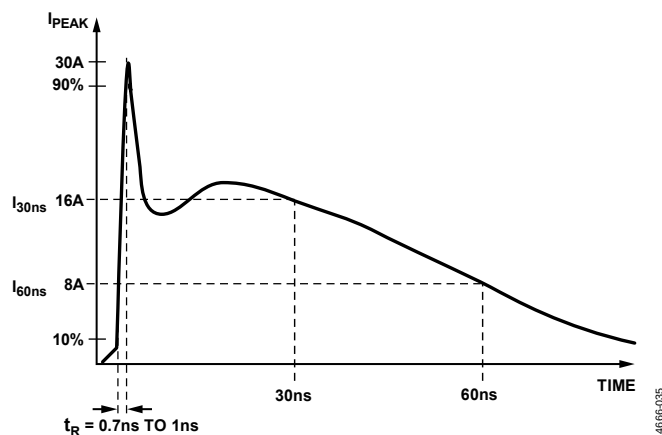
Figure 45. IEC 61000-4-2 ESD Waveform (8 kV)
