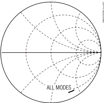
PCS-BAND MIXER S11
