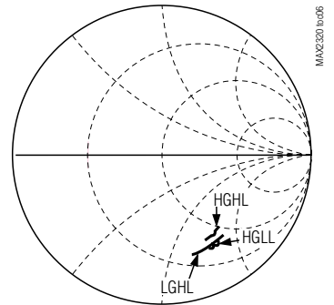
PCS-BAND LNA S22
