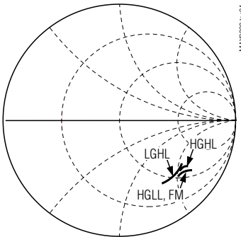
CELLULAR-BAND LNA S22
