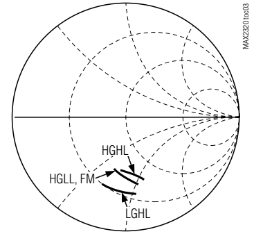
CELLULAR-BAND LNA S11
