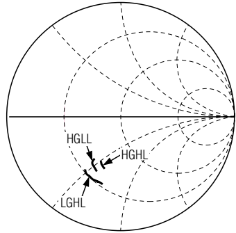
PCS-BAND LNA S11
