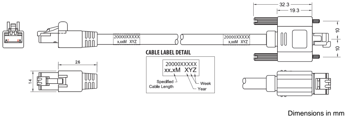
Fig. 1: Cable Overview
