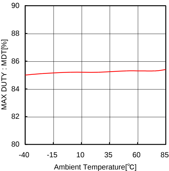
Figure 13. MAX DUTY vs Ambient Temperature
