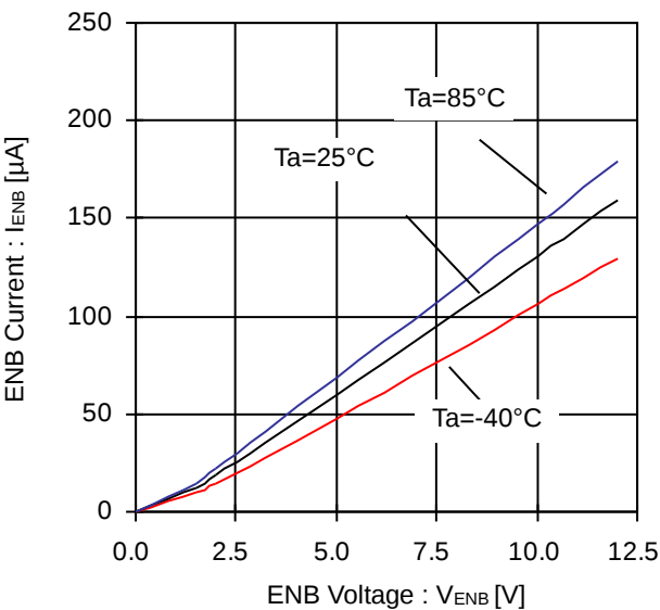
Figure 11. ENB Input Current vs ENB Voltage
