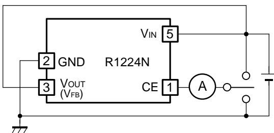
CE “H” Input Current, CE “L” Input Current
