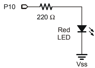
LED Indicator for Left IR Pair
