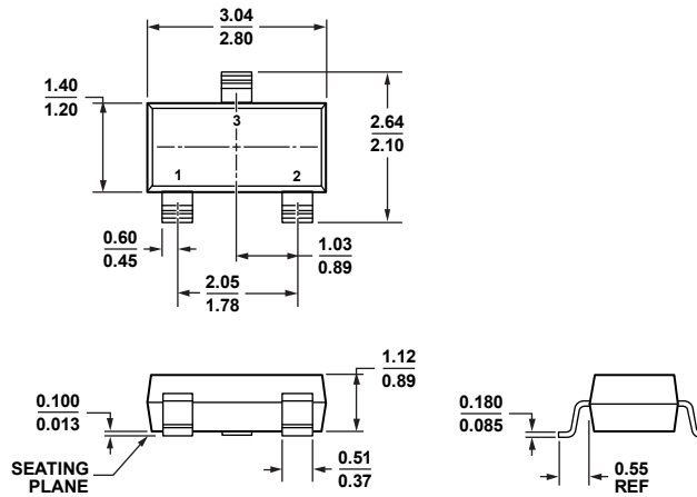
Figure 25. 3-Lead Small Outline Transistor Package [SOT-23-3] (RT-3)
