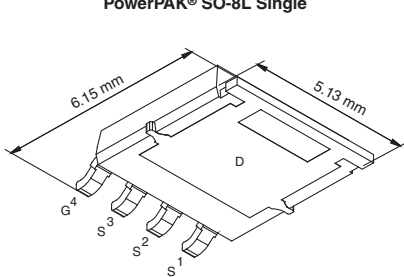
PowerPAK® SO-8L Single
