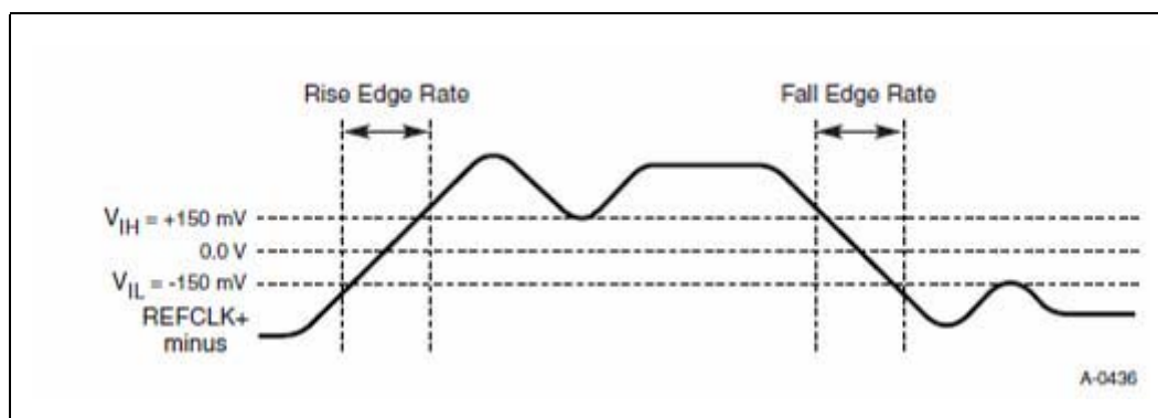
Figure 33-12. Differential Measurement Point for Rise and Fall Time
