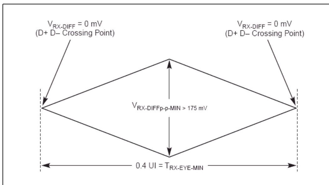
Figure 33-2. PCI Express Gen1 Receiver Eye
