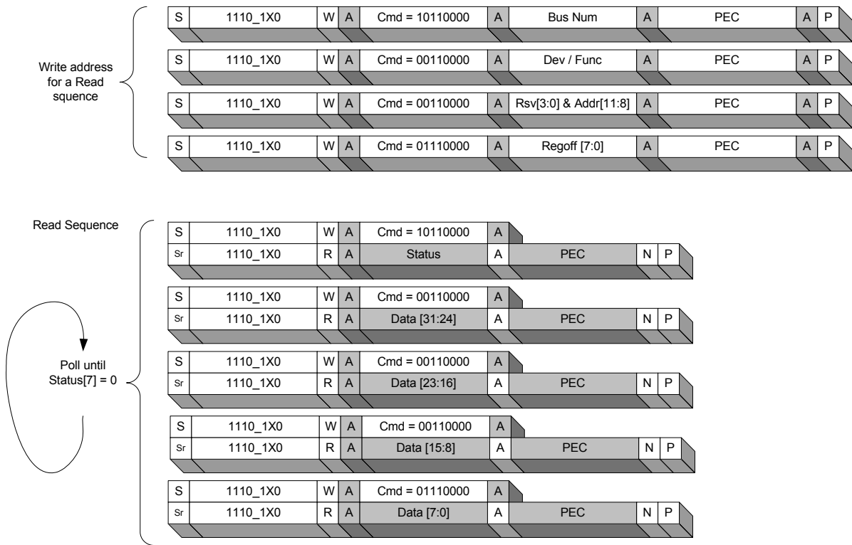
Figure 4-10. SMBus Byte-Size Memory Register Read
