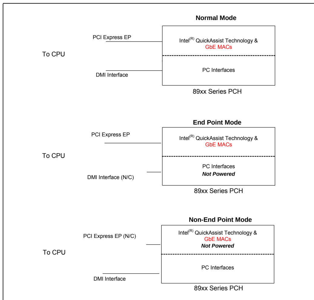
Figure 2-1. PCH Modes
