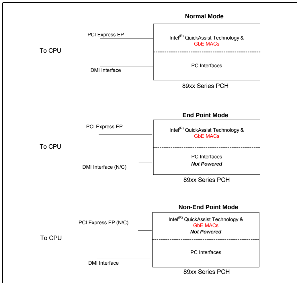
Figure 2-1. PCH Modes
