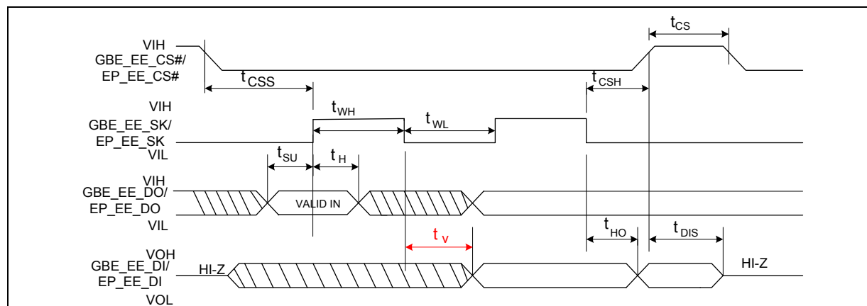
Figure 33-19. EEPROM Timing Diagram
