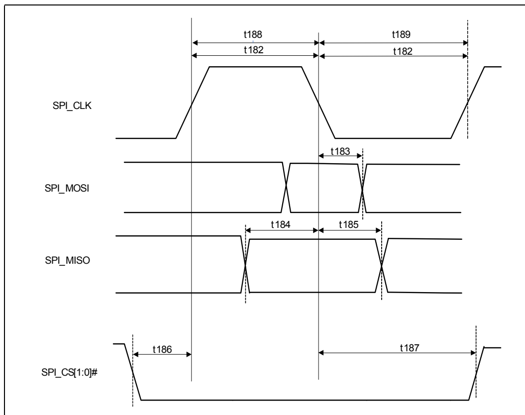
Figure 33-33.SPI Timings
