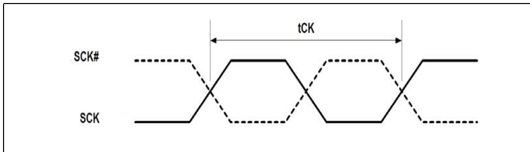
Figure 33-21.Clock Cycle Time
