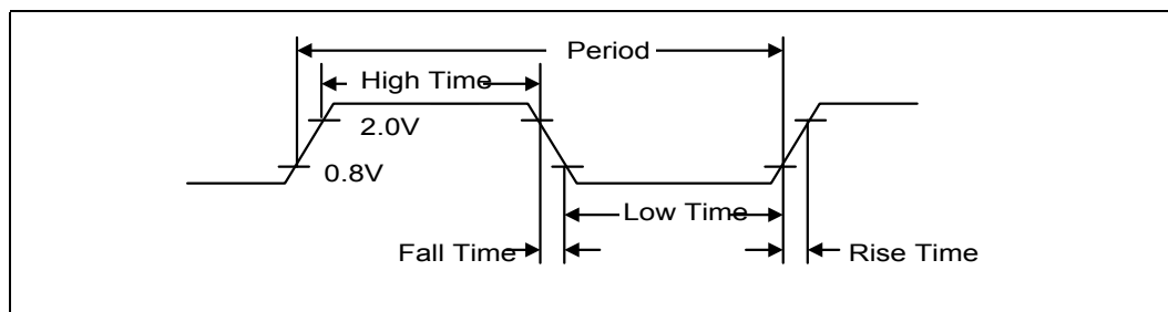
Figure 33-22. Clock Timing
