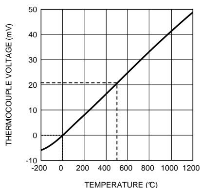
Figure 44. K-Type Thermocouple Response
