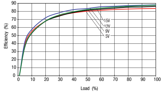
MEV1x24xxDC
