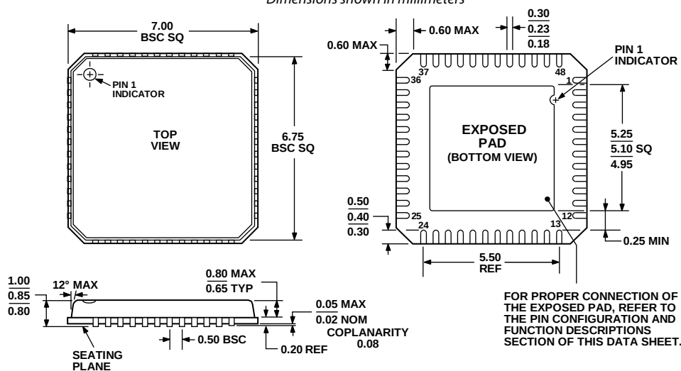
COMPLIANT TO JEDEC STANDARDS MO-220-VKKD-2 Figure 47. 48-Lead Lead Frame Chip Scale Package [LFCSP_VQ] 7 × 7 mm Body, Very Thin Quad (CP-48-1)
