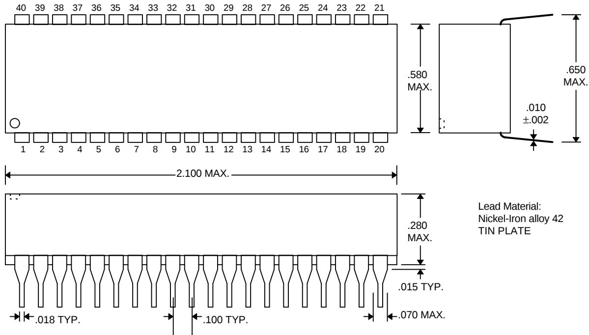
DIP (PDU17F-xx, PDU17F-xxM)
