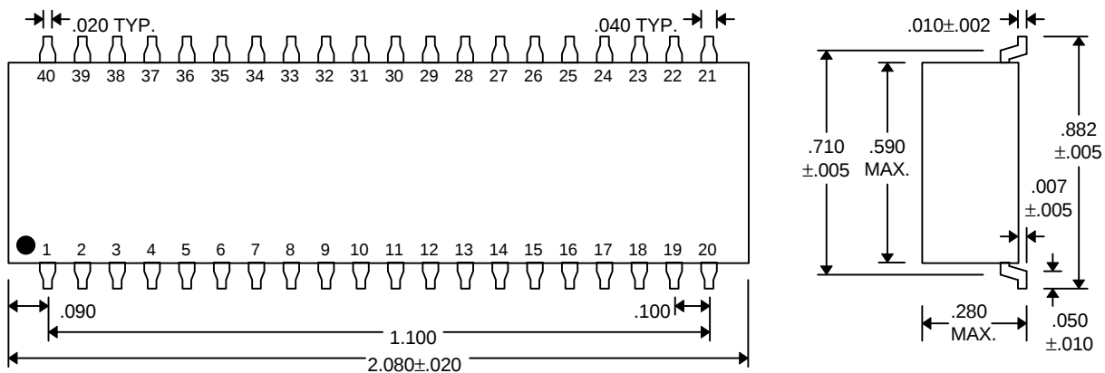
Gull-Wing (PDU17F-xxC5, PDU17F-xxMC5)
