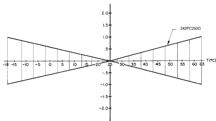
Null and Sensitivity Shift (% Span)
