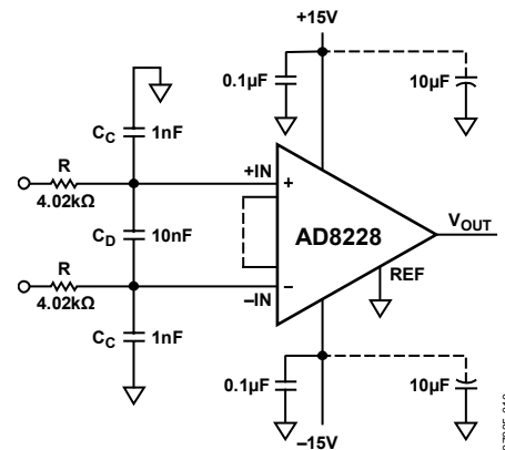
Figure 47. RFI Suppression
