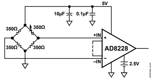
Figure 49. Precision Strain Gage
