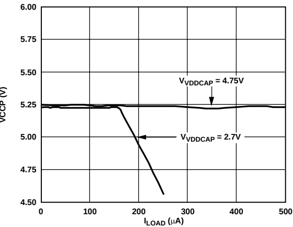
Figure 15. VCCP vs. Load Current
