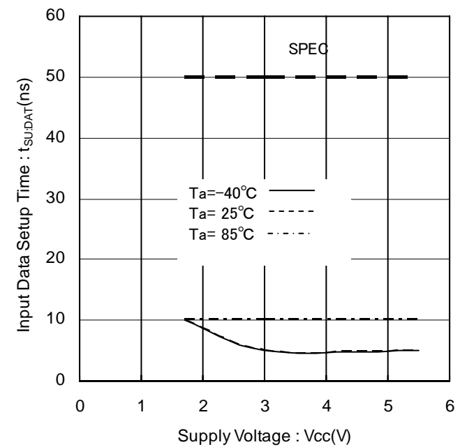
Figure 22. Input Data Setup Time vs Supply Voltage (LOW)
