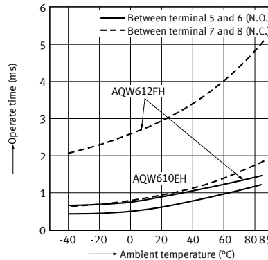
3. Operate time vs. ambient temperature characteristics
