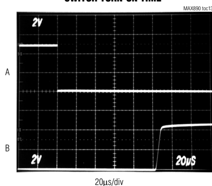
SWITCH TURN-ON TIME
