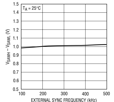
Oscillator ( V_{SAWH} - V_{SAWL} ) vs External Sync Frequency
