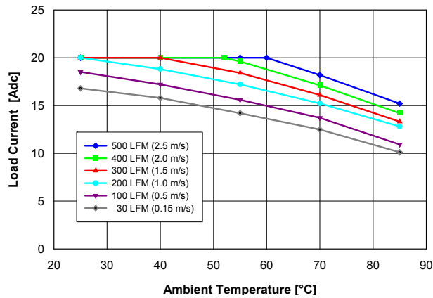
Fig. 1 : Available load current vs. ambient air temperature and airflow rates for converter with G height pins mounted vertically with air flowing from pin 1 to pin 3, MOSFET temperature \leq 125^{\circ}\text{C} , V_{in} = 48\text{ V} .
