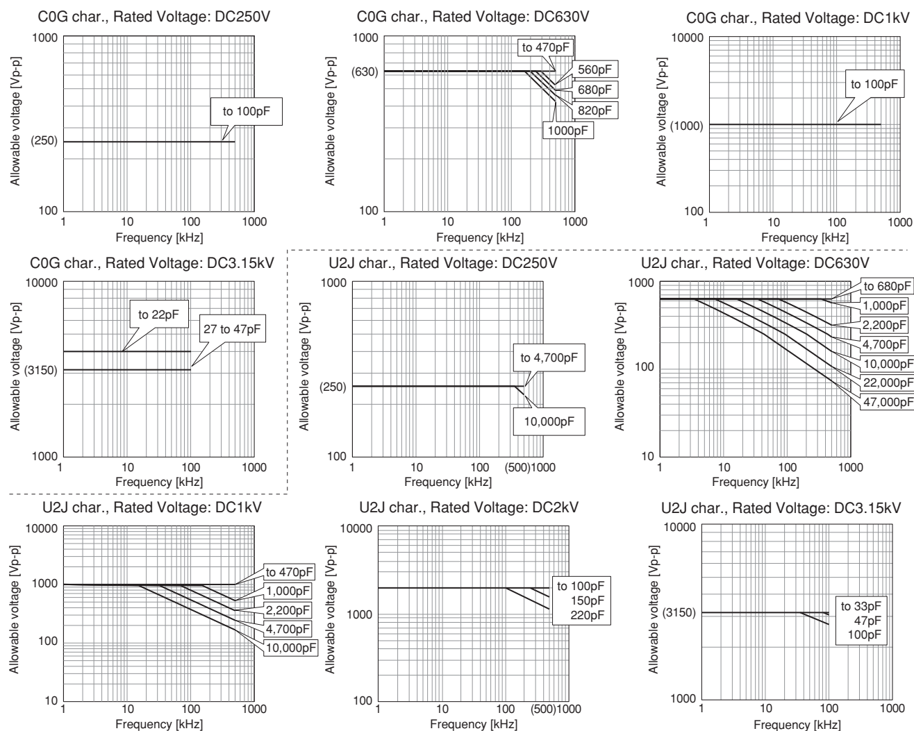
The sine-wave frequency VS allowable voltage
