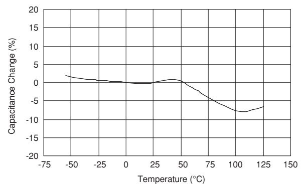
Typical Temperature Characteristics R7(X7R)
