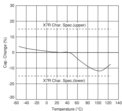
X7R Characteristics
