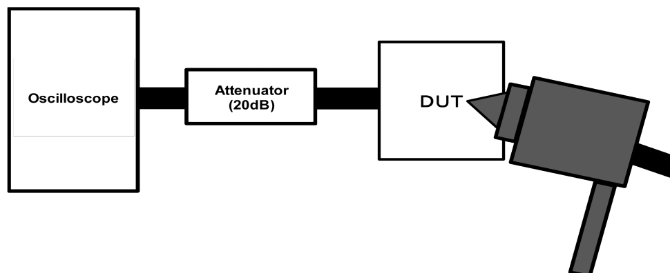
Fig. 10.3 IEC61000-4-2 (Contact)
