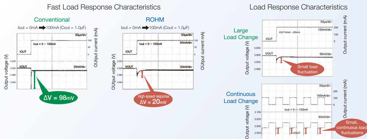
Figure 12. In general, in digital ICs, the current switches from 0 to I_{MAX} and vice versa, synchronized with the clock edge. During operation, if V_{OUT} suddenly drops below the operating range a malfunction could occur. ROHM's line of fast response CMOS LDOs combine a high (200 mA) current rating with exceptional dynamic load regulation.
