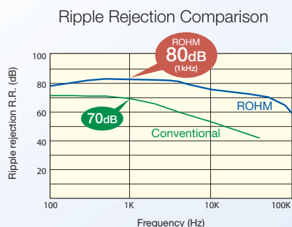
Figure 8. ROHM high ripple rejection LDOs provide rejection ratios of up to 80 dB without the need for the filter capacitors required with conventional regulators provide.
