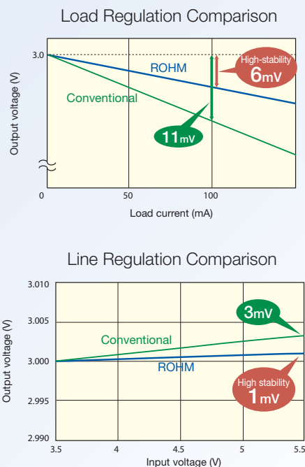
Figure 9. ROHM's proprietary circuitry assures power supply stability with significantly varying load currents or large input voltage variations.
