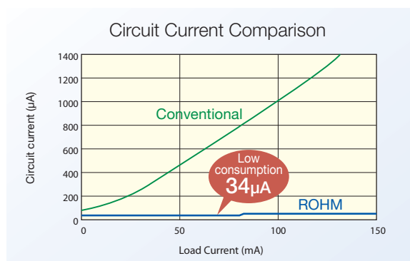
Figure 6. The P-channel MOSFET at the output stage of ROHM's line of Standard CMOS LDOs results in a dramatically lower circuit current than possible with convention bipolar types.
