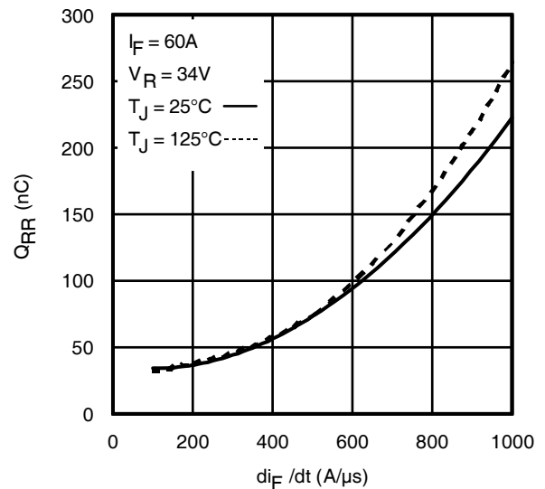
Fig. 20 - Typical Stored Charge vs. d i_F / d t
