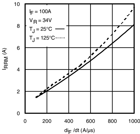
Fig. 19 - Typical Recovery Current vs. d i_F / d t
