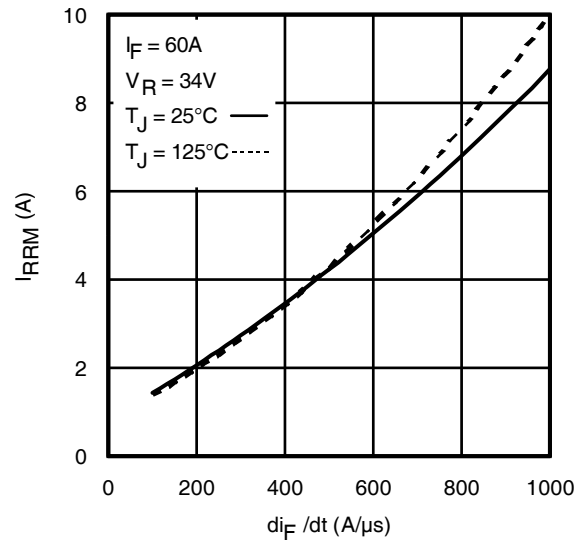
Fig. 18 - Typical Recovery Current vs. d i_F / d t
