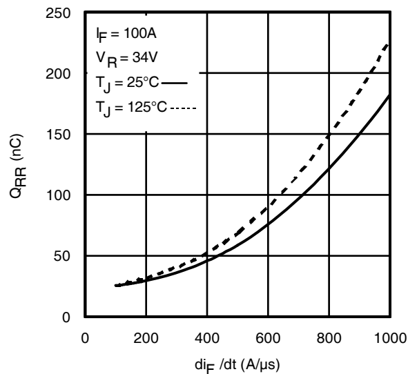
Fig. 21 - Typical Stored Charge vs. d i_F / d t
