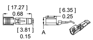
Open Barrel Contact
