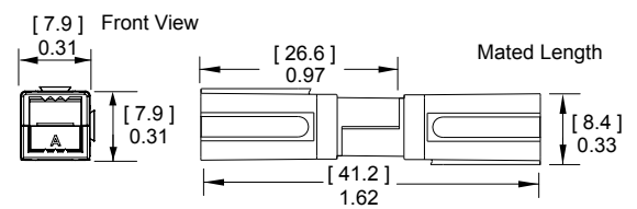
PP15-45 Finger Proof & Standard & Ground Housing Dimensions
