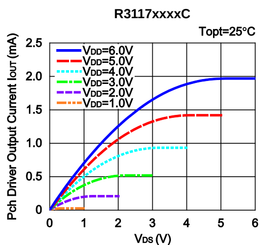
9) Pch Driver Output Current vs. V_{DS}
