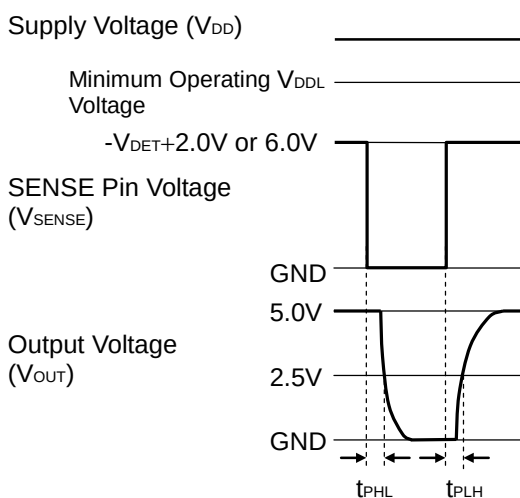
Nch Open Drain Output (R3117xxxA)
