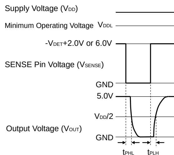
CMOS Output (R3117xxxC)
