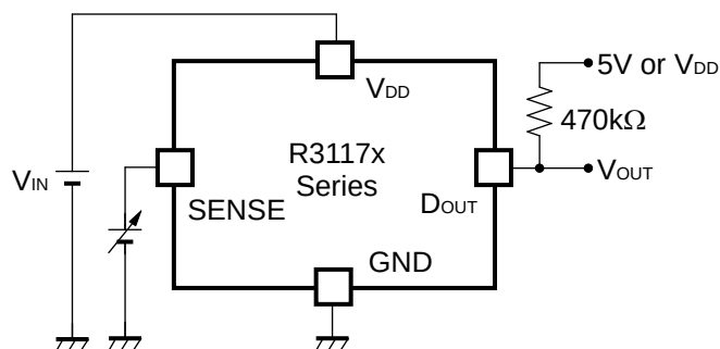
Detector Threshold Test Circuit (Pull-up circuit is not necessary for CMOS Output type.)
