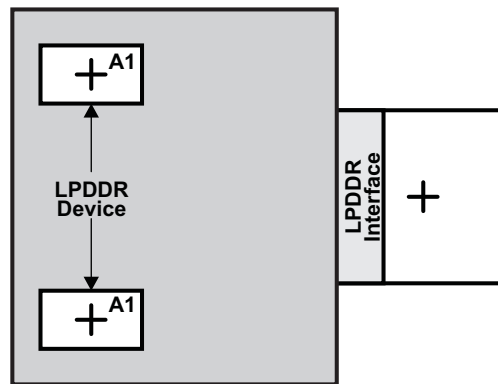
Figure 7-35. LPDDR Keepout Region
