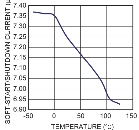
Soft-Start/Shutdown Current vs. Temperature
