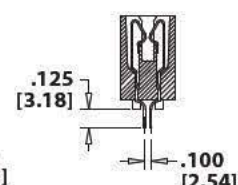
DIP SOLDER (HN)
