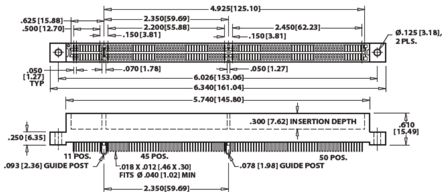
GBB106DHHD-S578, 106 (11/45/50) POSITIONS
