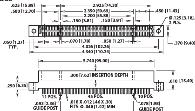
GBB66DHHD-S578, 66 (11/45/10) POSITIONS
