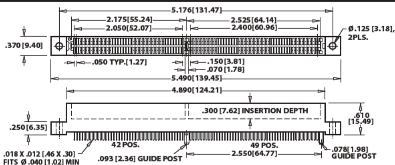
GBB91DHHD-S578, 91 (42/49) POSITIONS
