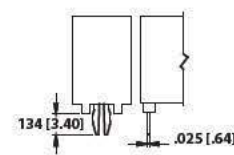
BOARD LOCK (R) (with no mounting ears)
