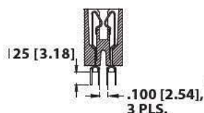
STAGGERED DIP SOLDER (HH)
