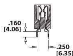
DIP SOLDER (HL)
