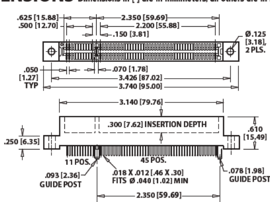
GBB56DHHD-S578, 56 (11/45) POSITIONS
