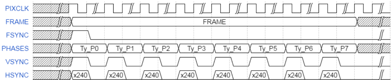
Figure 5 : FSYNC, VSYNC & HSYNC timing diagram 1
