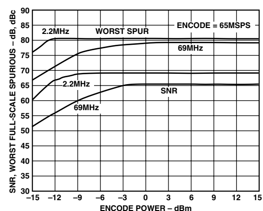
TPC 12. SNR, Worst Spurious vs. ENCODE Power
