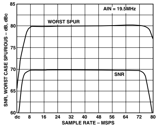
TPC 10. SNR, Worst Spurious vs. ENCODE
