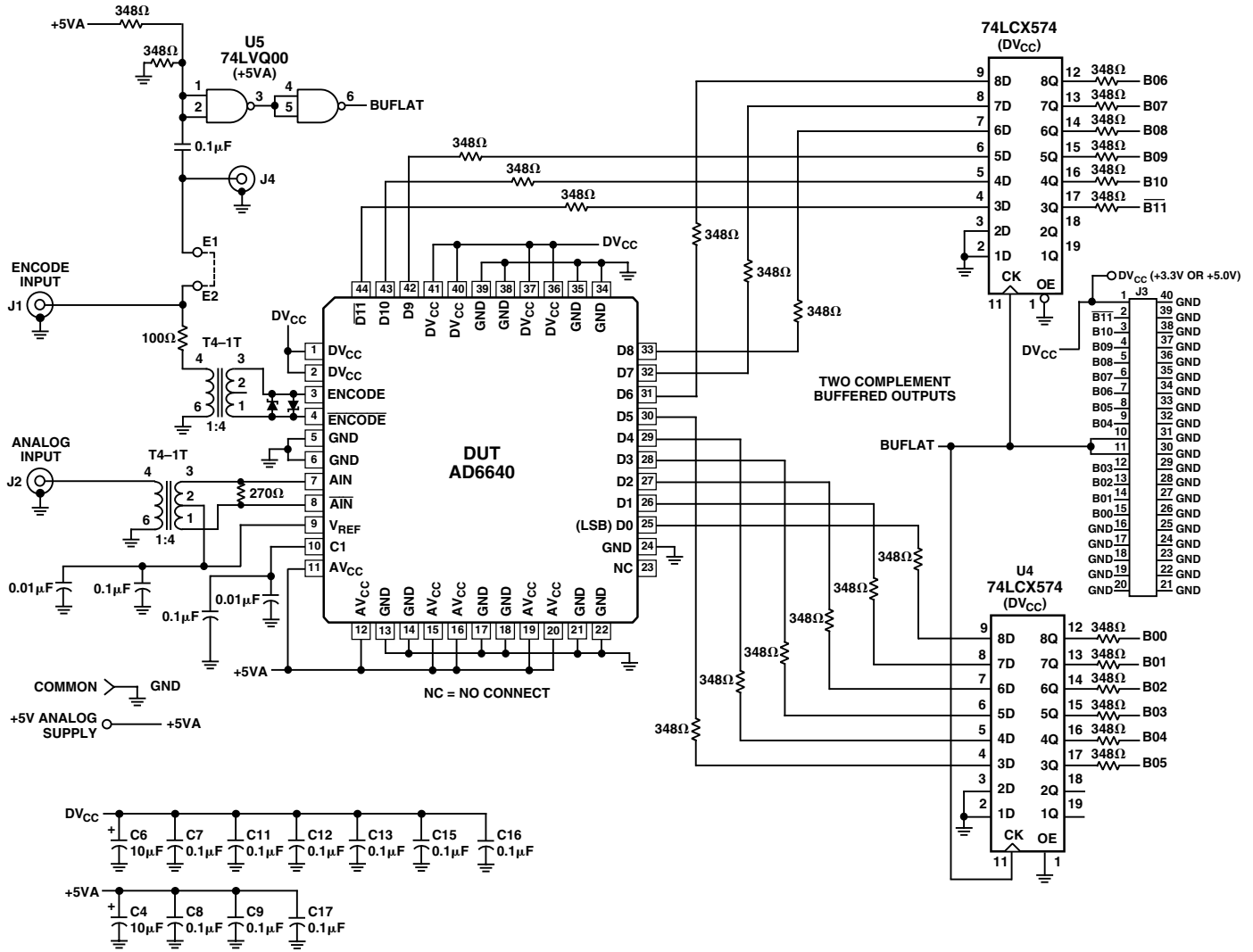
Figure 18. AD6640ST/PCB Schematic
